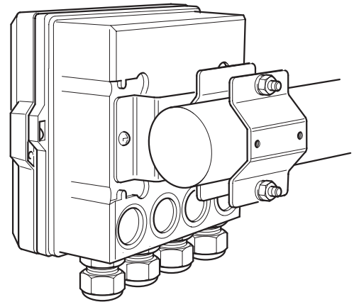
Horizontal pipe-mount
