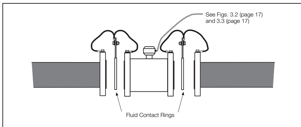
Fig. 3.1 Grounding – All Pipes
