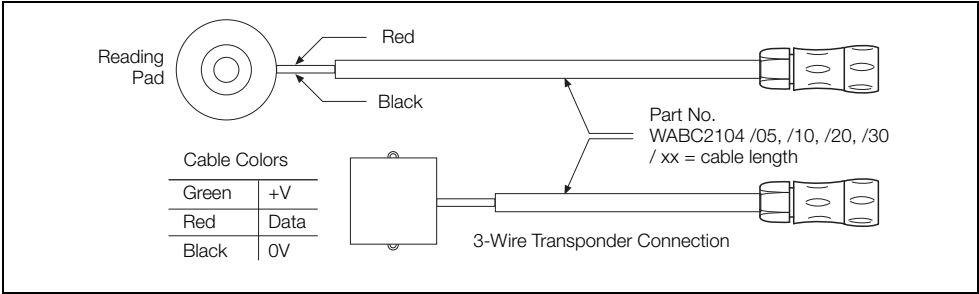
Fig. 3.9 ScanReader Connections
