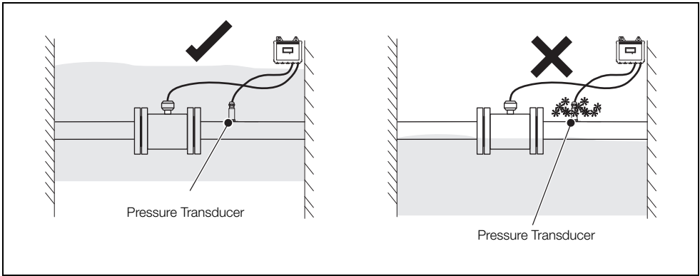
Fig. 2.18 Pressure Transducer – Protect from Frost
