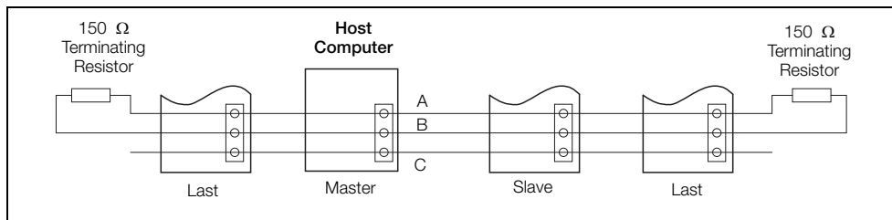
Fig. 3.16 Termination Resistor Location
