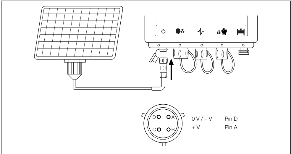
Fig. 3.19 Connecting a Renewable Energy Supply
