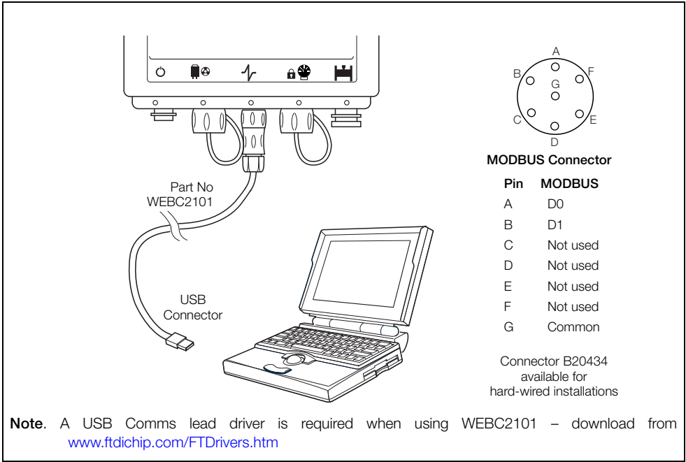
Fig. 3.13 MODBUS Connection
