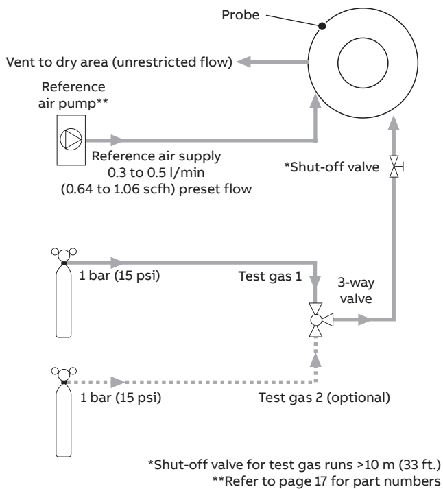
Non-AutoCal with test gas(es) and restrictors
