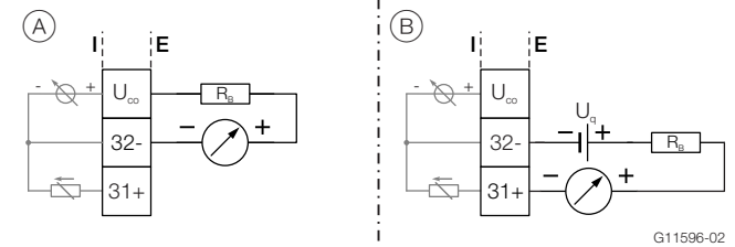
Fig. 28: (I = internal, E = external, R B = load, U q = Source voltage)
