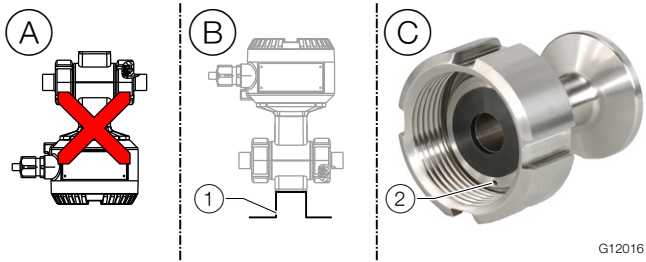
Fig. 16: 3A-compliant installation
