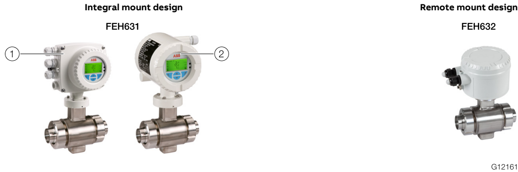
Fig. 2: Designs (example, devices with variable process connections)
