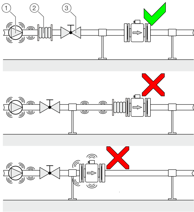
Fig. 14: Vibration damping
