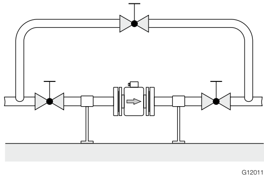
Fig. 3: Bypass connection
