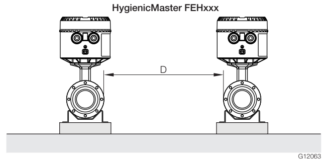
Fig. 2: Minimum distance
