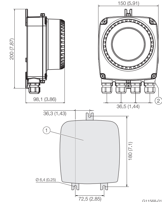
Fig. 26: Mounting dimensions single-compartment housing
