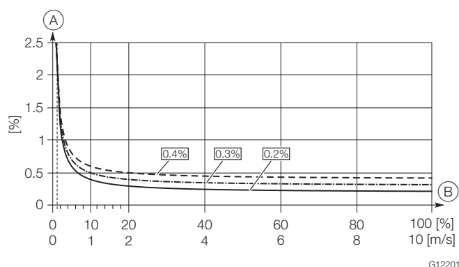
Fig. 5: Measuring error
