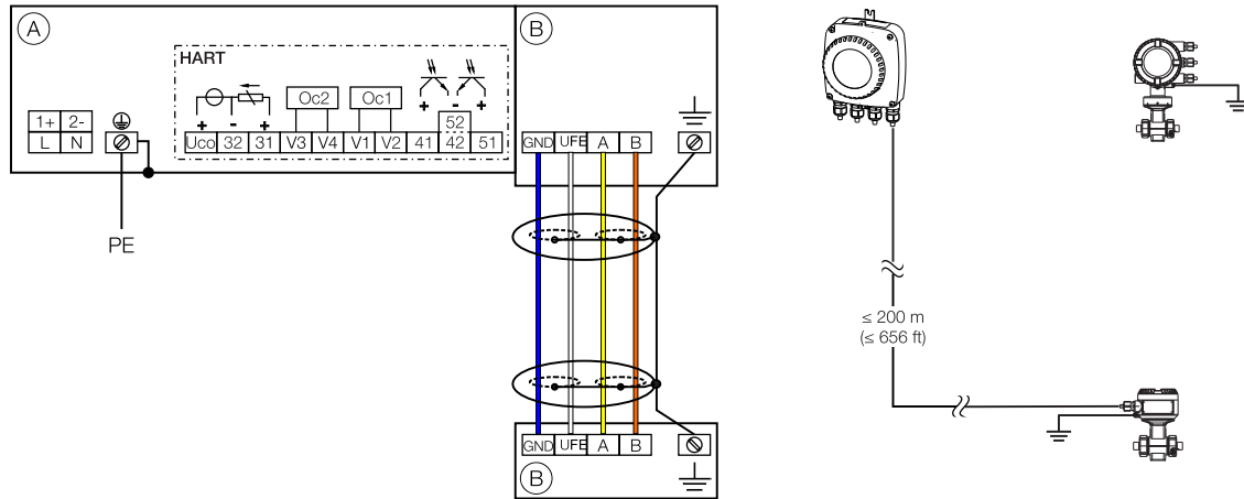
Fig. 27: Electrical connections
