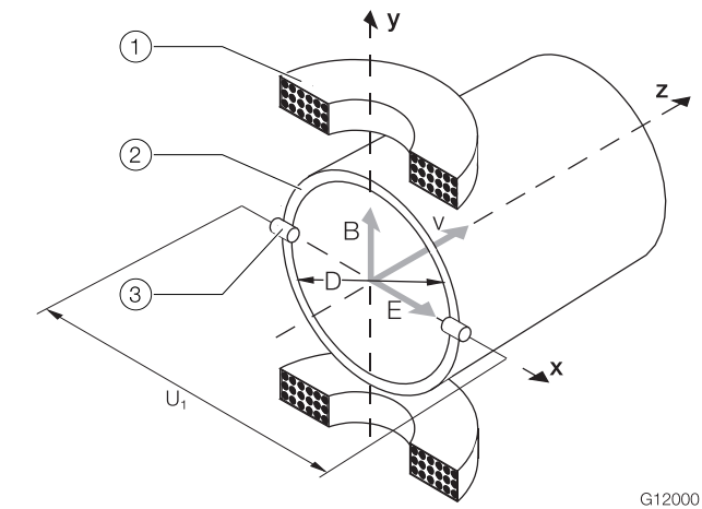
Fig. 4: Electromagnetic flowmeter schematic
