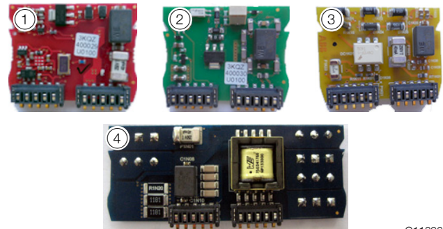
Fig. 25: Optional plug-in cards
