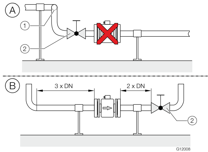
Fig. 12: In- and outlet section, turn-off component
