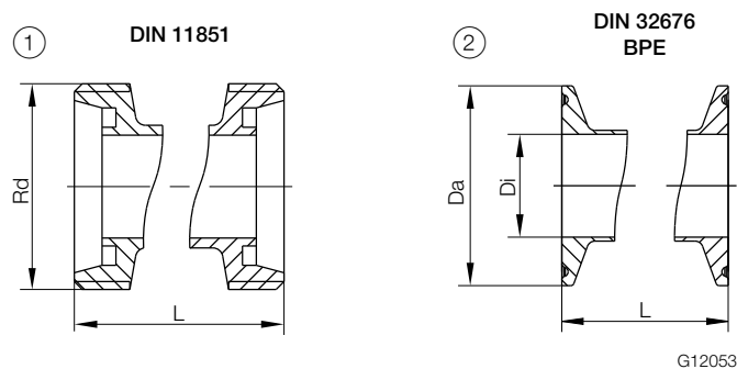
② Tri-Clamp
