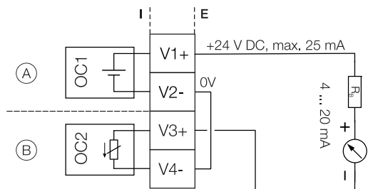
Fig. 39: Active current output V3 / V4 (example)
